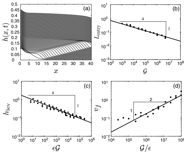
FIG. 2. (a) The evolution of a peeling front obtained by solving (7) and (8). Successive profiles are shifted vertically (thus time increases from bottom to top in the plot). (b) The entry length L_{\text{entry}} as a function of the dimensionless hydrostatic pressure \mathcal{G} ; the line is the scaling law (9). (c) The levitation height h_{\text{lev}} as a function of \epsilon\mathcal{G} ; the line is the scaling law (10). (d) The velocity of the peeling front v_f as a function of \mathcal{G}/\epsilon ; the line is the scaling law (11). In each case, the points correspond to the results of numerical simulations of (7) and (8). In (d), points deviate from the predicted scaling at small \mathcal{G} where the assumption that hydrostatic effects dominate breaks down.
