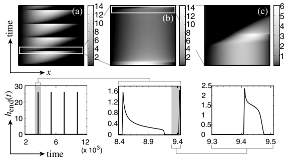
FIG. 4. (a) Top panel shows an alternative representation of the data in Fig. 3(a). Grey scale indicates gap thickness and time increases along the vertical axis. The sharp horizontal lines illustrate the rapid time scales associated with gap closure. The bottom panel shows the vertical position of the end of the membrane as a function of time. (b) Expanded view of the white box in (a) and associated time series for the vertical position of the end of the membrane illustrating venting. Time has been shifted by t_{\text{shift}} = 2500 to coincide with the first spike in (a). (c) Expanded view of the white box in (b) showing healing. Time has again been shifted by t_{\text{shift}} = 2500 . The membrane zips shut from left to right expelling fluid.
