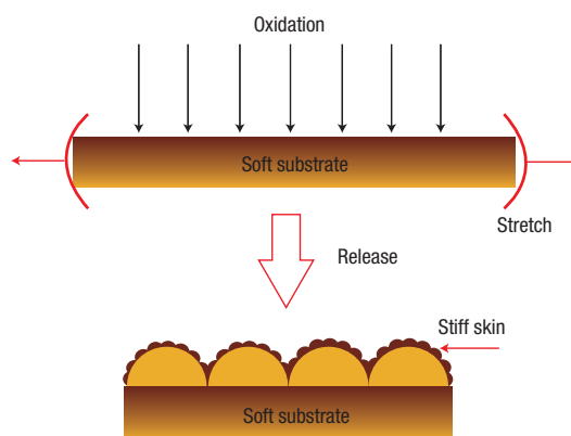
Figure 1 Experimental procedure for preparing nested wrinkles. A thin, stiff SiO 2 skin is formed on a stretched elastomeric (PDMS) substrate by UV oxidation. Release of the substrate causes the skin to wrinkle. As the strain is released further, the skin buckles again and again until the strain is completely removed.
