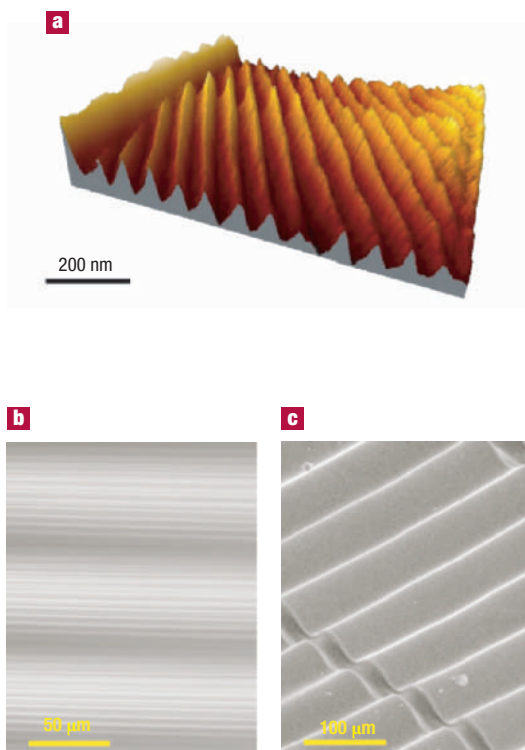
Figure 2 Nested wrinkling patterns. a , Scanning force microscope image of first-generation ( \sim 50 nm wavelength) wrinkles. b,c , Optical microscopy images of third generation ( b , \sim 5 \mu\text{m} wavelength) and fourth generation ( c , \sim 50 \mu\text{m} wavelength) wrinkles.
